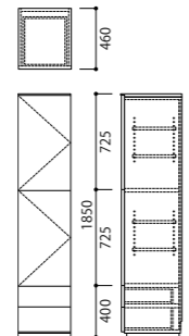
SBH-□2801R-HK2 (右開き扉)
