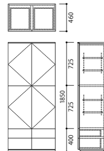
SBH-□2801R-HK2 (右開き扉)
