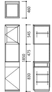
SBH-□2881L (左開き扉)
