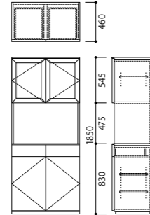
SBH-□2881L (左開き扉)
